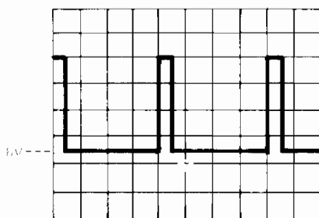
7 1 V/DIV 5 ns/DIV
