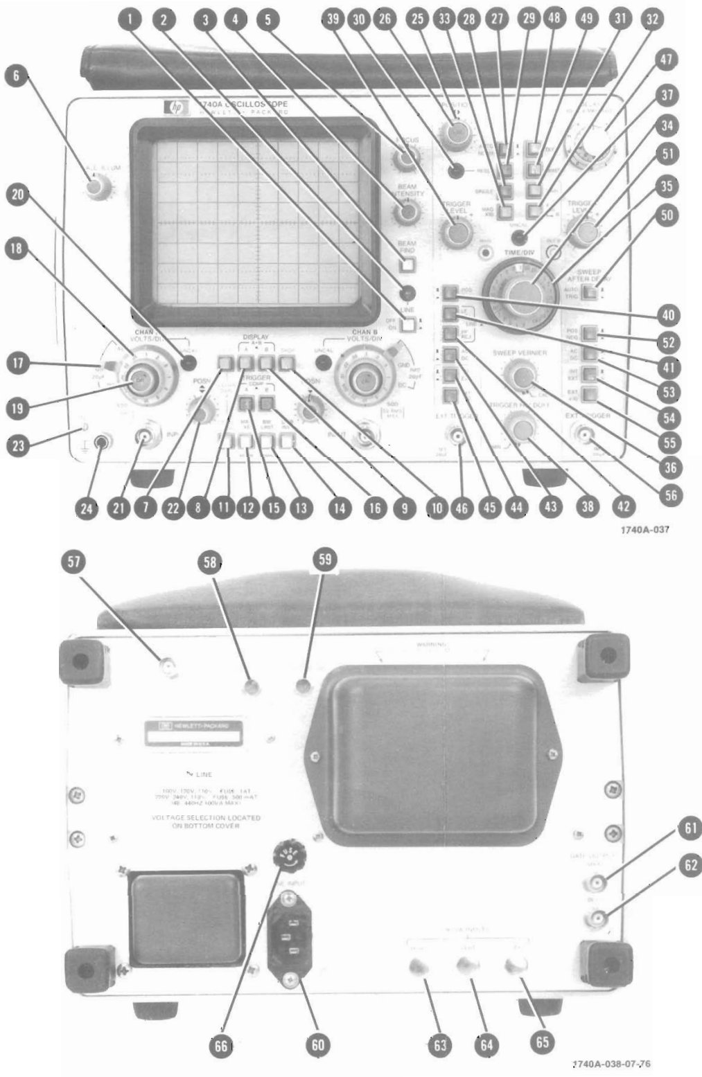
Figure 3-1. Controls and Connectors 3-0
