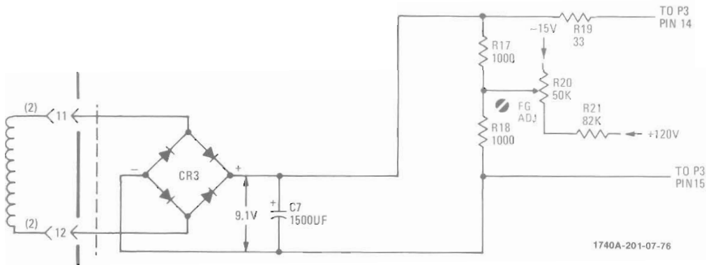
Figure 7-5. Changes to Schematic 1
