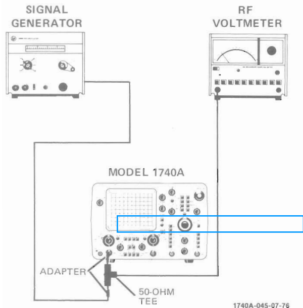
Figure 5-1. Bandwidth Test Setup
