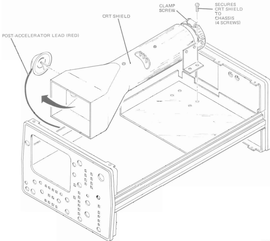
Figure 8-2. CRT Removal
