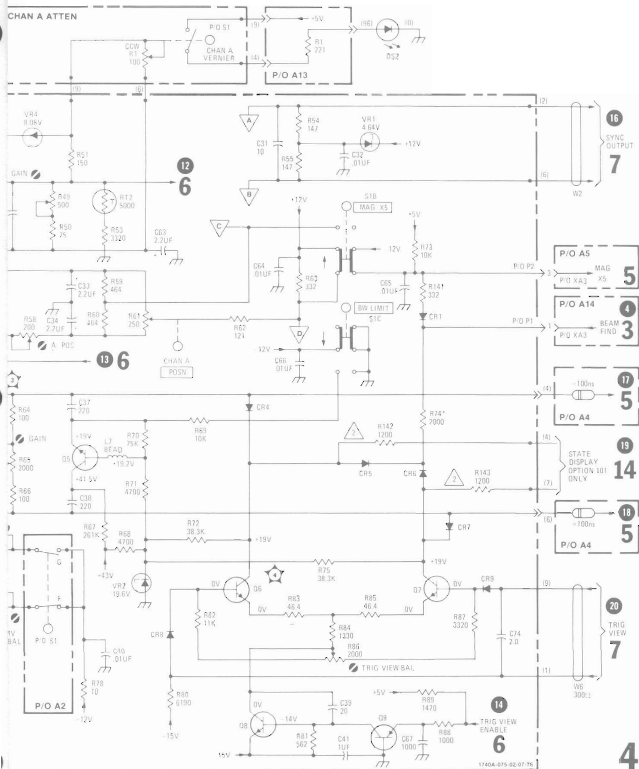
Figure 8-13. Service Information, Vertical Preamplifier Assembly A3 (Sheet 2 of 2)
