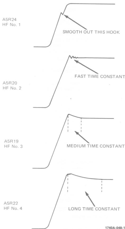
Figure 5-4. Pulse Response Adjustments
