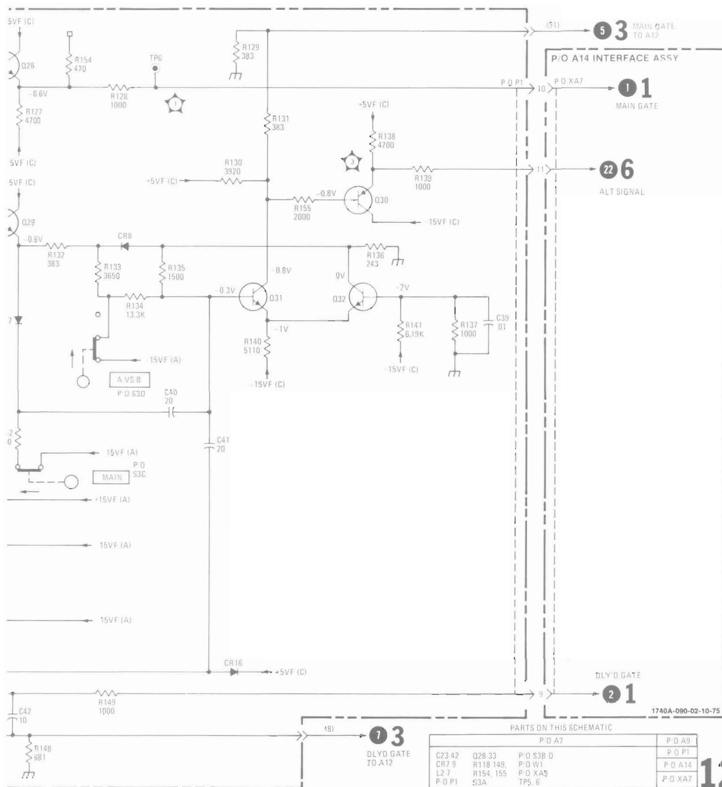
Figure 8-21. Service Information, Gate Schmitt, P/O Assembly A7 (Sheet 2 of 2) 8-35/(8-36 blank)
