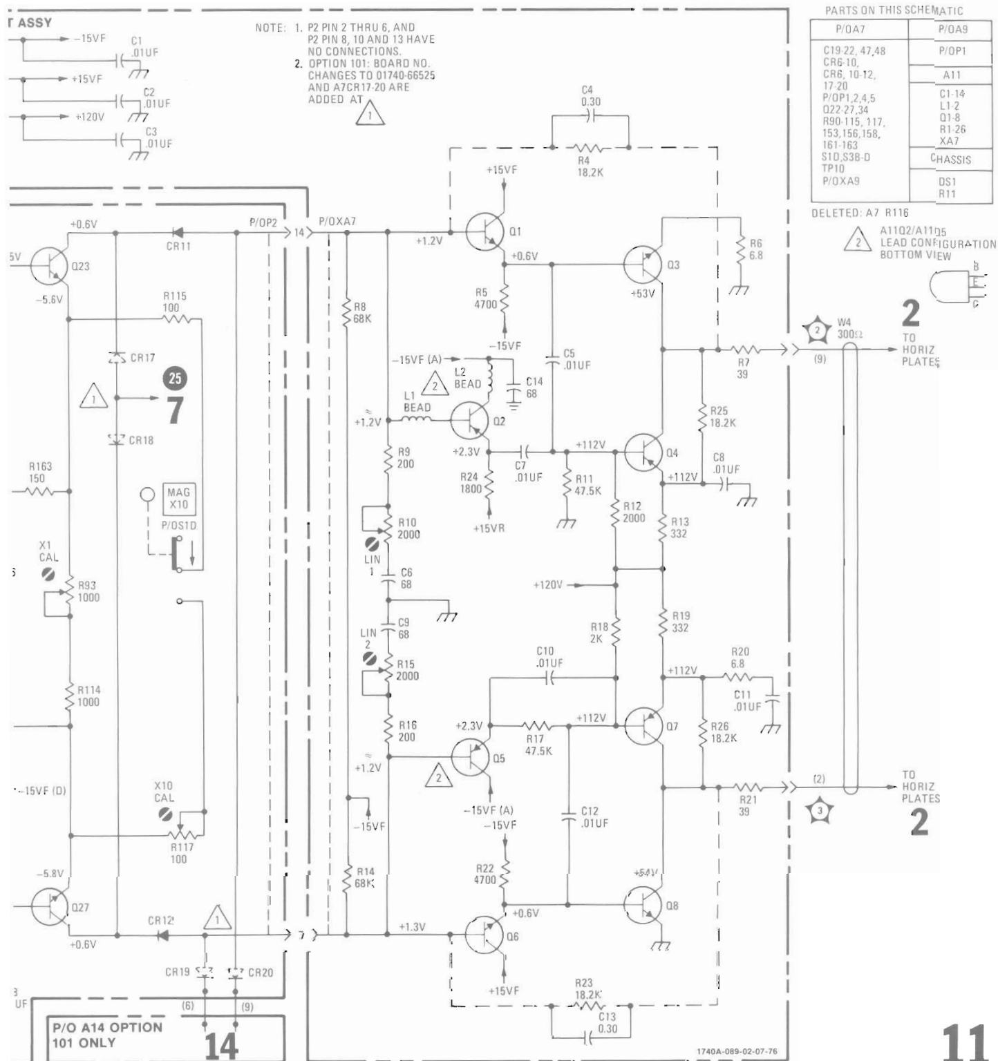
Figure 8-20. Service Information, Horizontal Output Assembly A11 and Horizontal Sweep Assembly A7 (Sheet 2 of 2) 8-33
