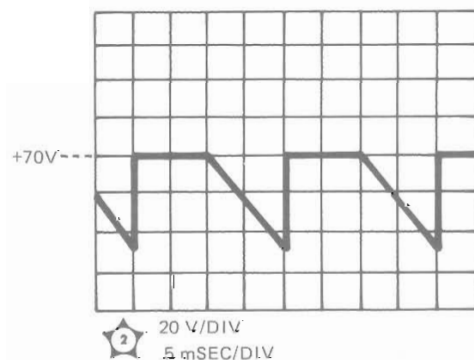
Figure 8-20. Service Information, Horizontal Output Assembly A11 and Horizontal Sweep Assembly A7 (Sheet 1 of 2)
