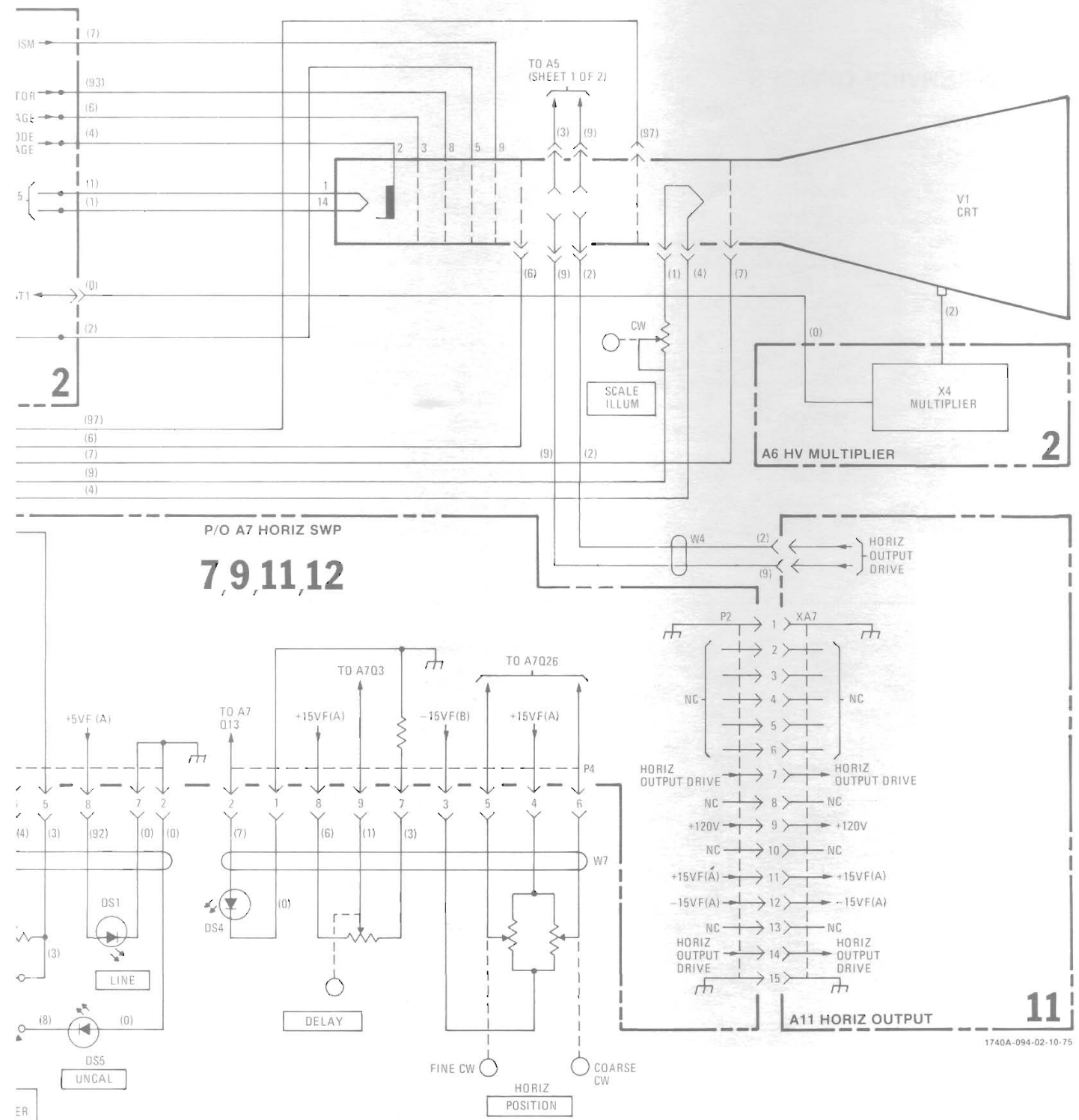
Figure 8-24. Interconnection Diagram (Sheet 2 of 2) 8-41
