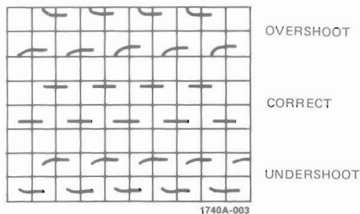
Figure 3-2. Probe Compensation
