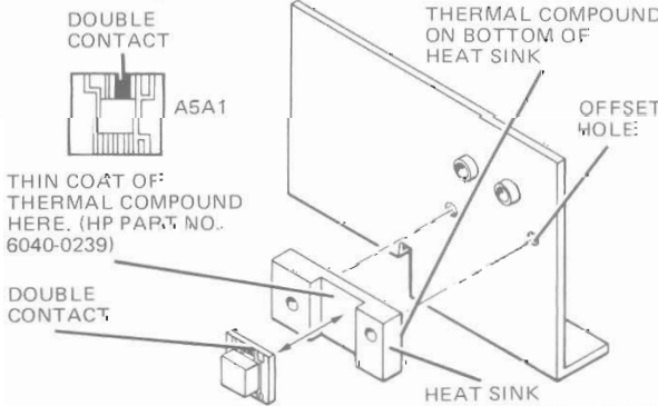
Figure 8-6. A5A1 Removal
