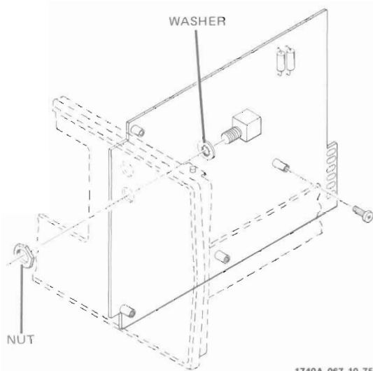
Figure 8-8. Location of A7 Attaching Screws
