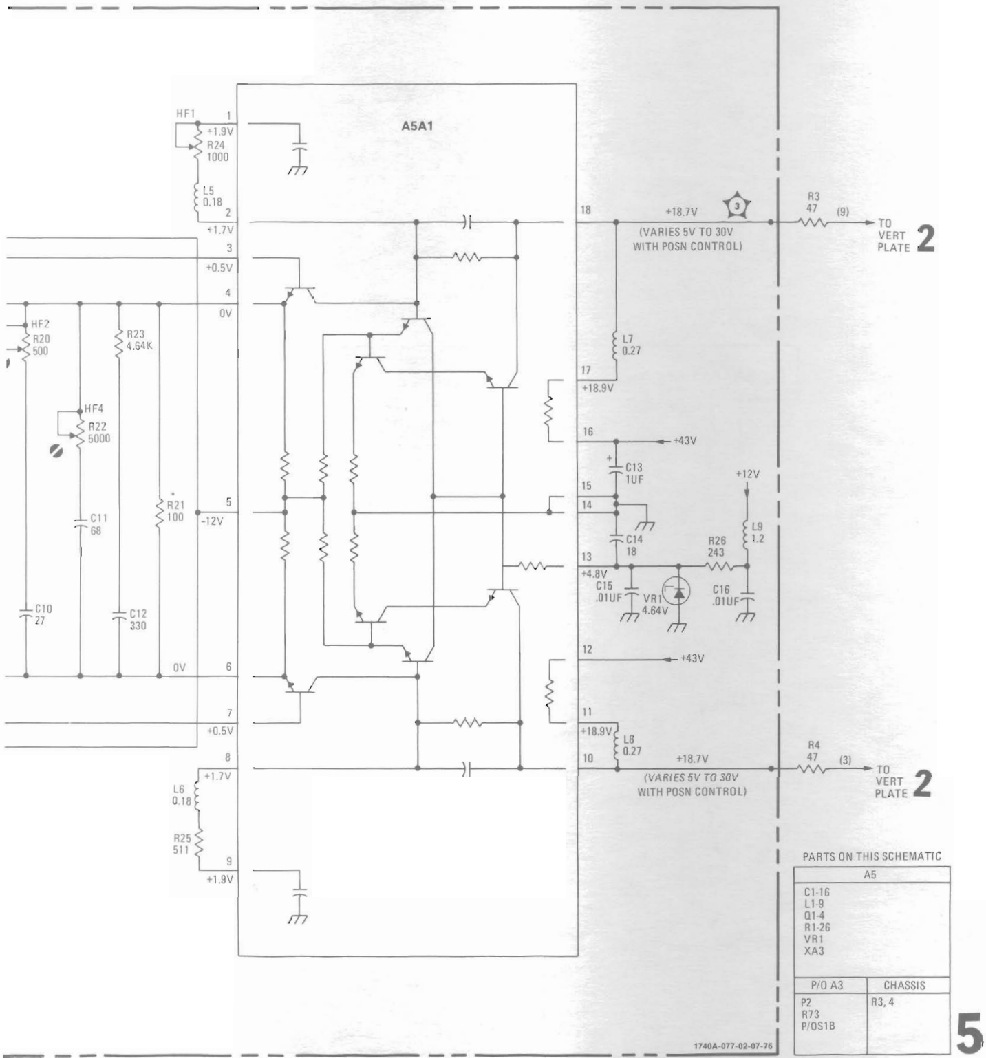
Figure 8-14. Service Information, Vertical Output Assembly A5 (Sheet 2 of 2) 8-21
