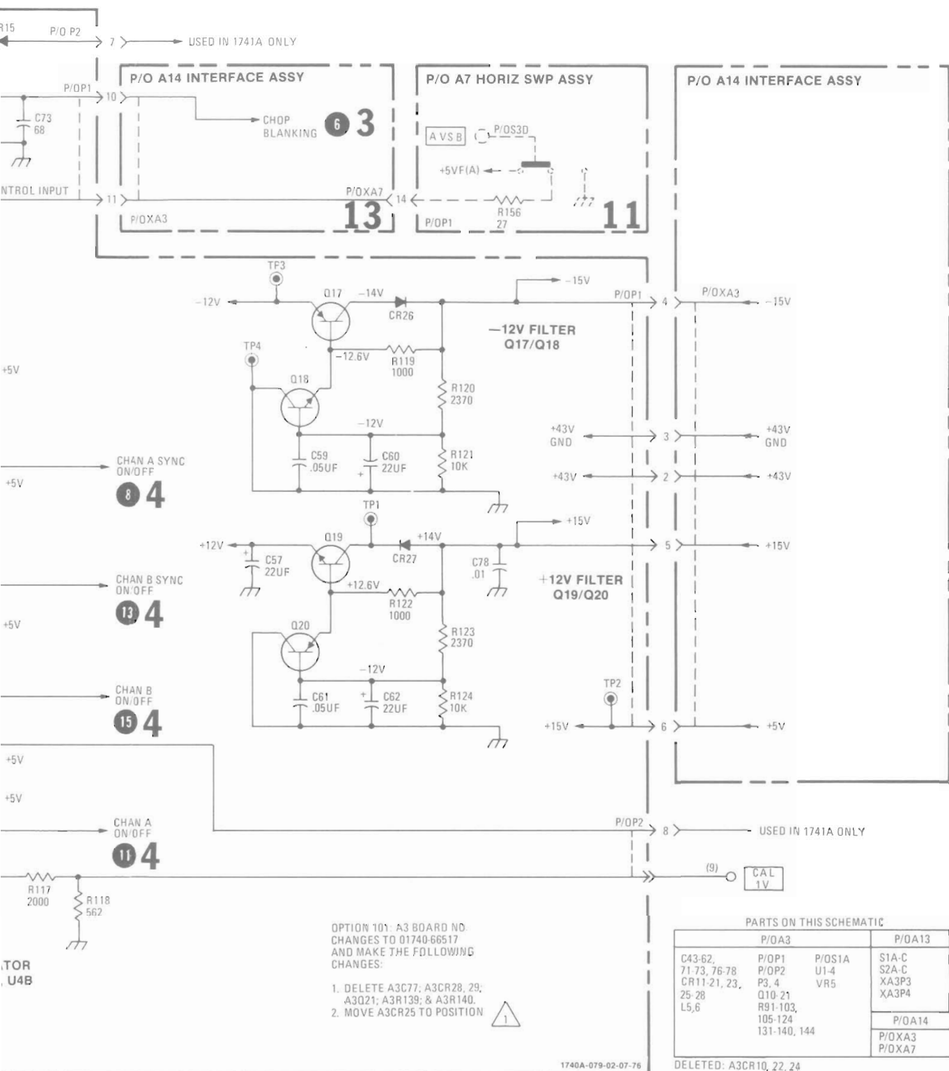
Figure 8-15. Service Information, Vertical Control Switching Assembly A13 and Vertical Preamplifier Assembly A3 (Sheet 2 of 2) 8-23
